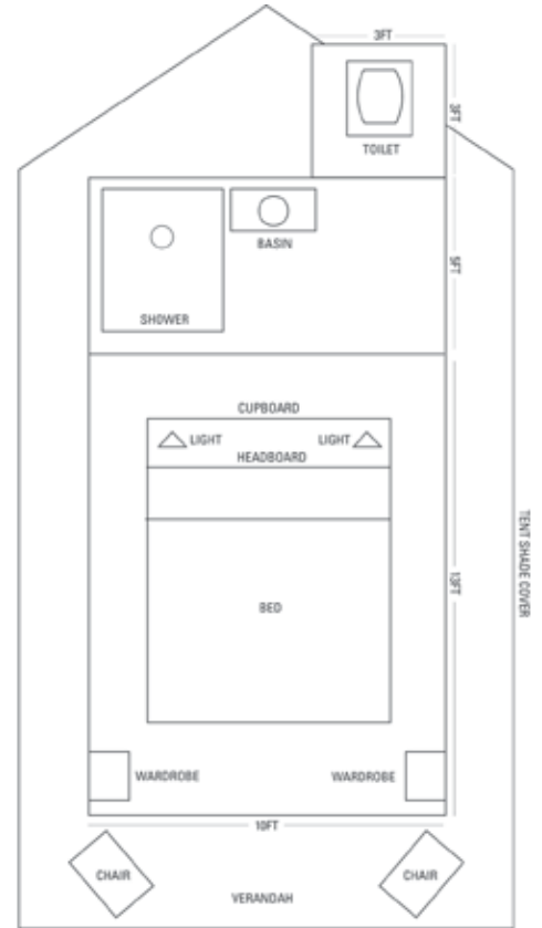
MOBILE TENT LAYOUT 10' X 18'
