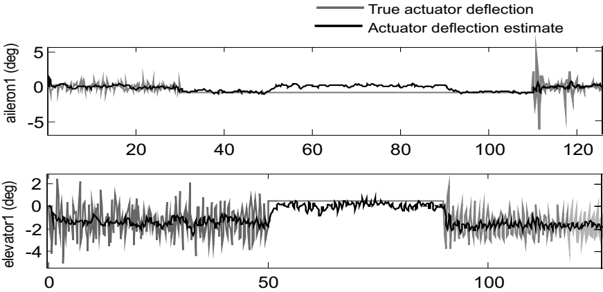
Fig. 4.28 Estimation of the deflection of the faulty control surfaces
