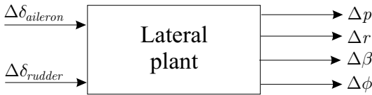
Fig. 8.1 Linear model of the aircraft lateral-directional motion
