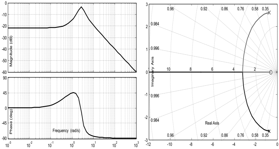
Fig. 8.11 Bode plot and root locus of the channel \dot{r}_{des} to r_{meas} with uncertainty levels indicated in (8.24) to (8.27)
