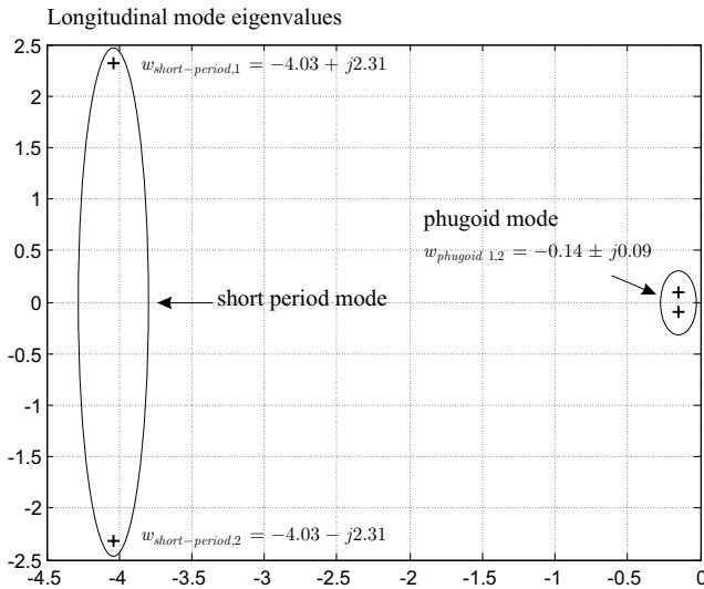
Fig. 7.2 Aircraft longitudinal mode eigenvalues
