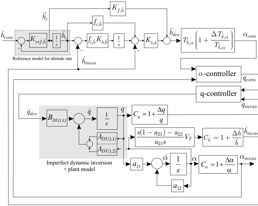
Fig. 7.28 Rate-of-climb controller
