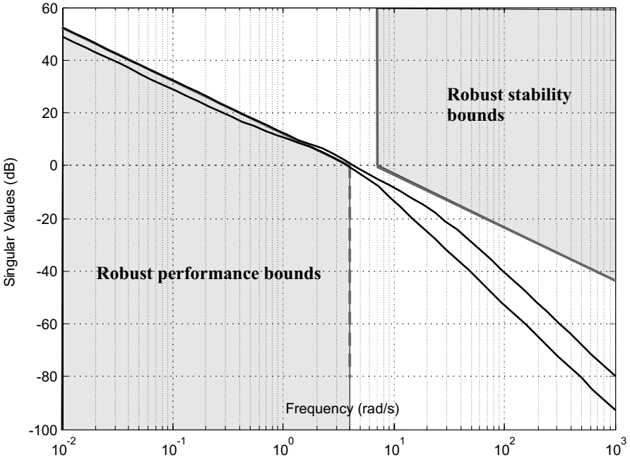
Fig. 8.17 SVs of the loop gain G_1 K_1 , with uncertain dynamic inversion of the plant by 30% uncertainty level on each variable according to (8.24) to (8.27). k_{b,roll}=22 [s^{-1}] and K_{b,yaw}=23 [s^{-1}]
