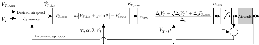
Fig. 7.36 Nonlinear airspeed controller
