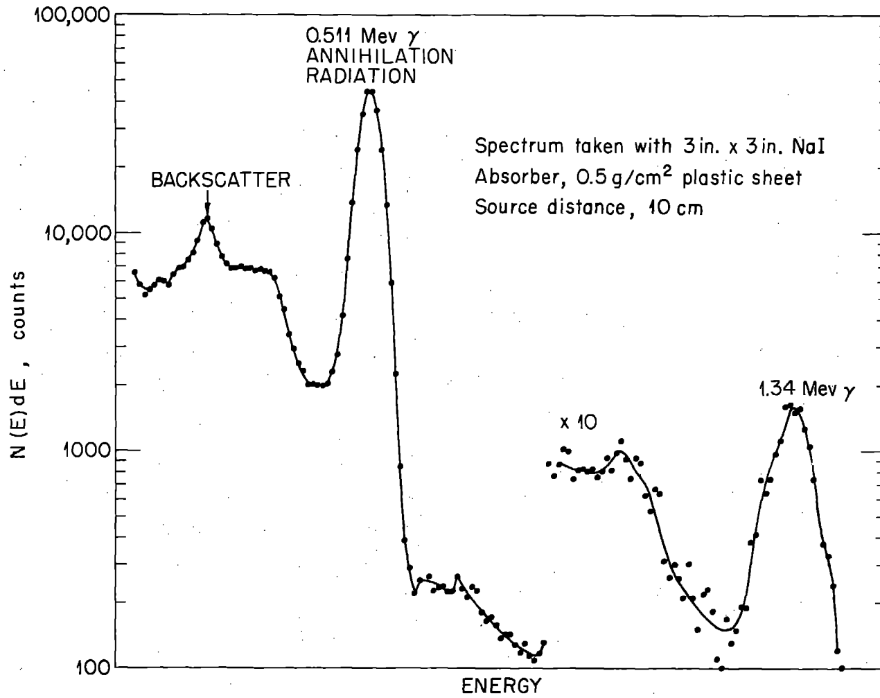
Fig. 4 Gamma-ray spectrum of \text{Cu}^{64} , half-life = 12.8 hr.
