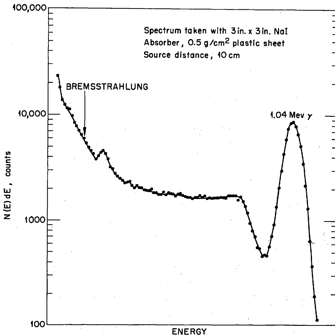
Fig. 6. Gamma-ray spectrum of \text{Cu}^{66} , half-life = 5.1 min.
