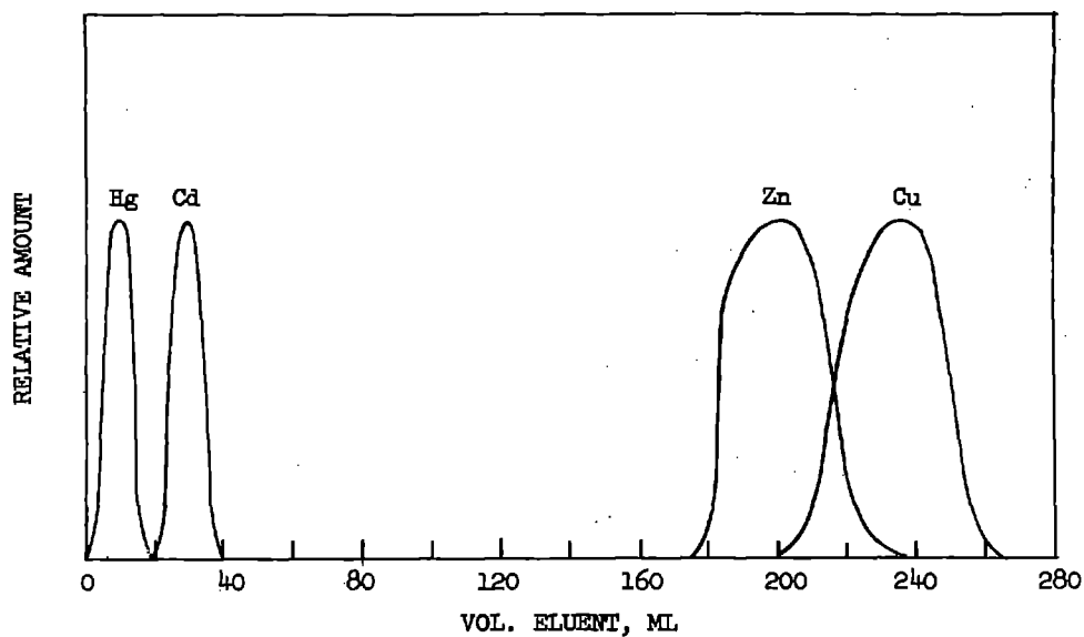
Figure 2. Elution curves for some of the divalent metal ions; 3.1 M HCl used as eluent; ion exchange resin, Dowex 50, 200-400 mesh. (Taken from UCRL-2531. (82) )
