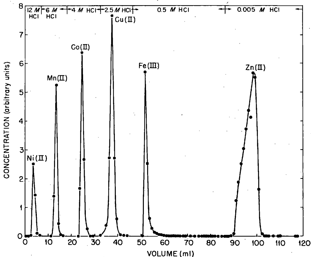
Figure 3. Separation of Transition Elements Mn to Zn. (Dowex-1 Column; 26 cm x 0.29 cm., flowrate = 0.5 cm/min.). Taken from Kraus, K. A. and Moore, G. E., J. Am. Chem. Soc. , 75 , 1460 (1953).
