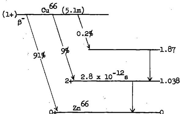
Figure 5. Decay Schemes of Copper-64 and Copper-66. Taken from Strominger, D., Hollander, J. M., and Seaborg, G. T., Rev. Modern. Phys. 30 , 585-903 (1958).
