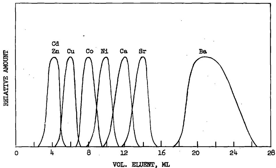
Figure 1. Elution curves for some of the divalent metal ions; 3.1 M HCl used as eluent; ion exchange resin, Dowex 50, 200-400 mesh. (Taken from UCRL-2531. (82) )
