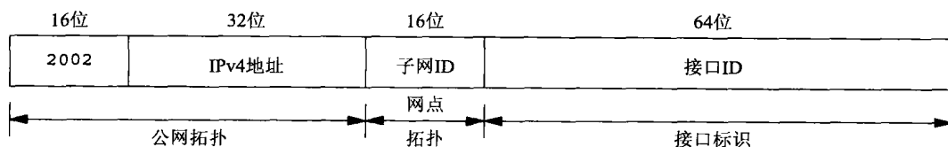
图B-3 6to4地址
