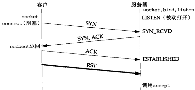
图5-13 ESTABLISHED状态的连接在调用accept之前收到RST
