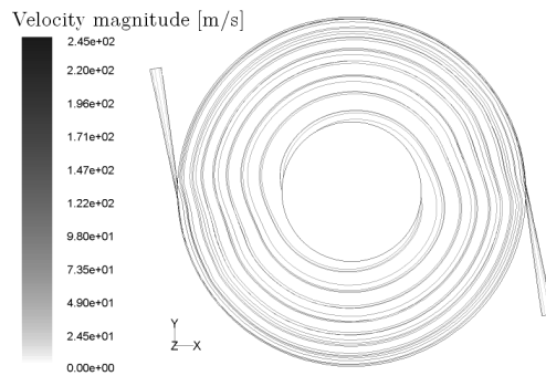
Fig. 11. Pathlines coloured by velocity magnitude; 2 supply nozzles, disk diameter 300 mm, inlet angle 10^\circ ; rotational speed 9 000 rpm
