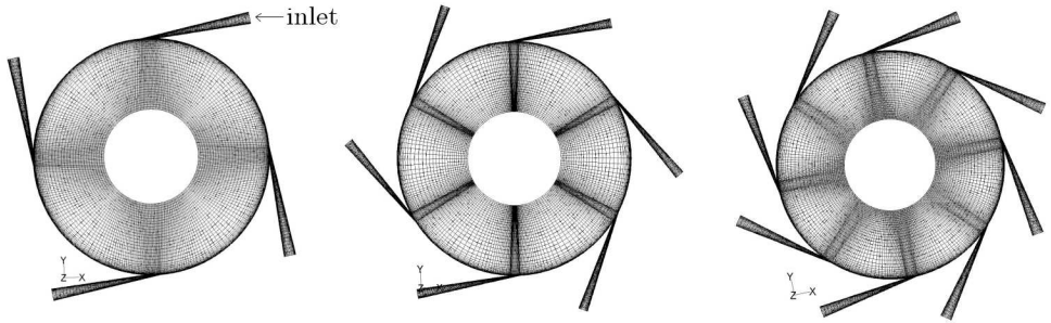
Fig. 3. Calculation domain for three different nozzle configurations of the simplified model of a Tesla turbine
