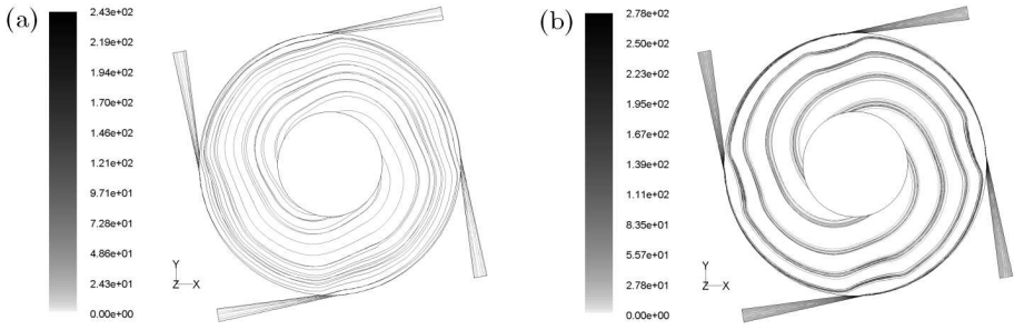
Fig. 7. Pathlines distinguished by the velocity magnitude at nominal load, disk diameter 100 mm, inlet angle 10^\circ ; (a) 18 000 rpm, (b) 9 000 rpm
