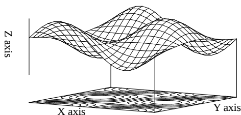
3D surface with projected contours
