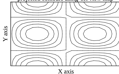
projected contours using 'set view map'
