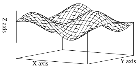
3D surface plot with hidden line removal
