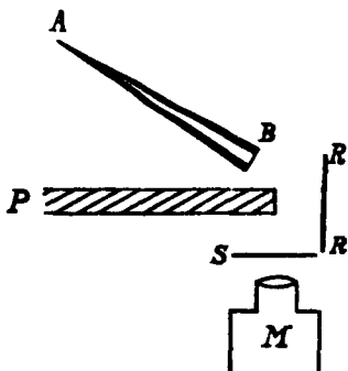
Arrangement of Ernest Marsden's experiment: A-B, alpha particle source. R-R, gold foil. P, lead plate. S, zinc sulfide scintillation screen. M, microscope.
