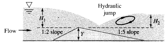
Fig. P10.122 The Crump weir [19, chap. 4]
