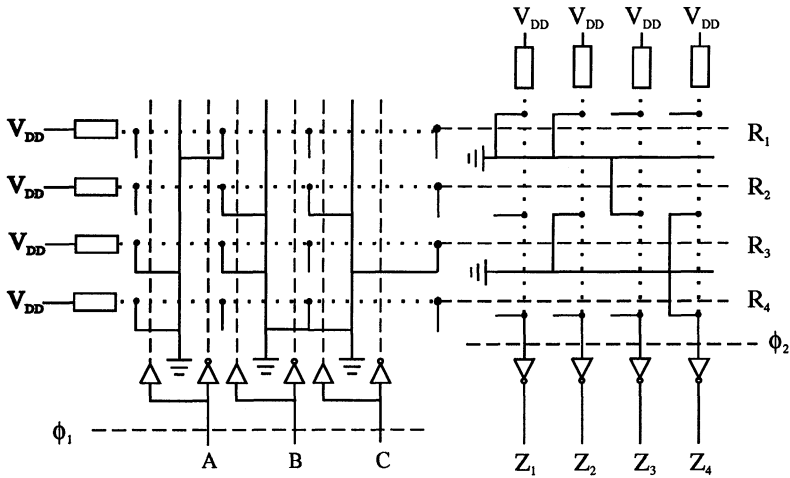
Fig. 7.54 Circuit Diagram for a PLA
