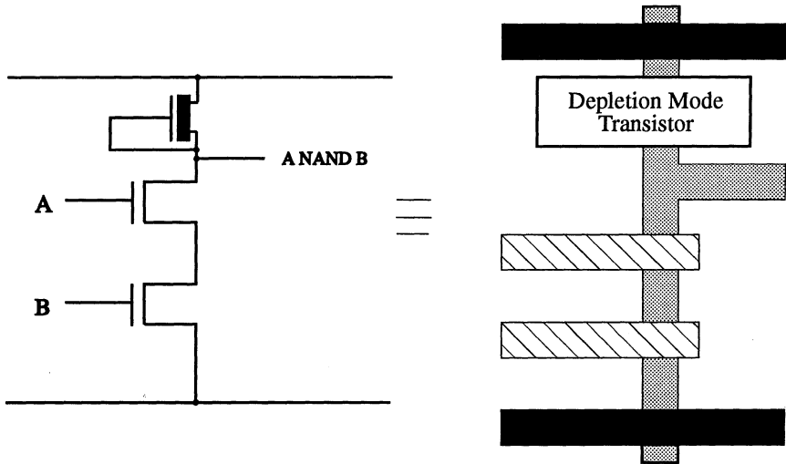
Fig. 7.43 The NAND Gate
