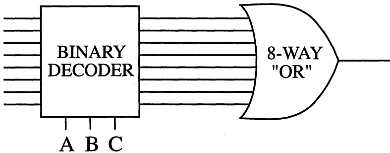
Fig. 2.17 The Multiplexer
