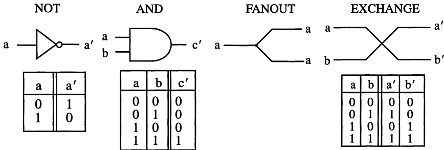
Fig. 6.1 Primitive Elements
