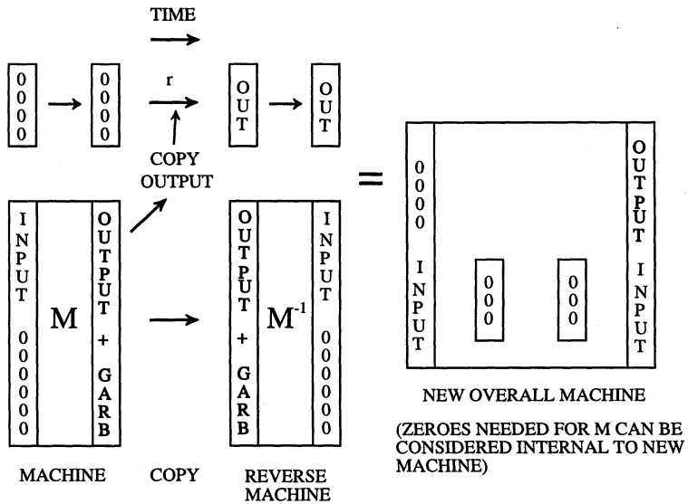
Fig. 6.6 Clearing Garbage
