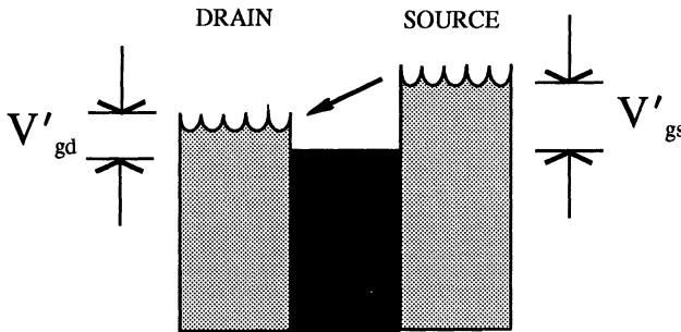
Fig. 7.9 Fluid Analogy for the Forward-Biased MOSFET
