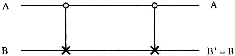
Fig. 2.21 The Identity Utilizing CN Gates
