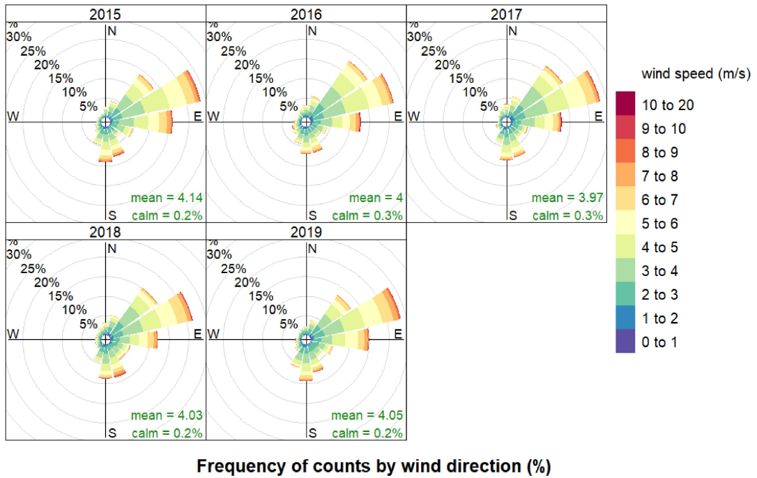
Figure A2 Annual distributions of winds at Blackwater (BoM) 2015 to 2019
