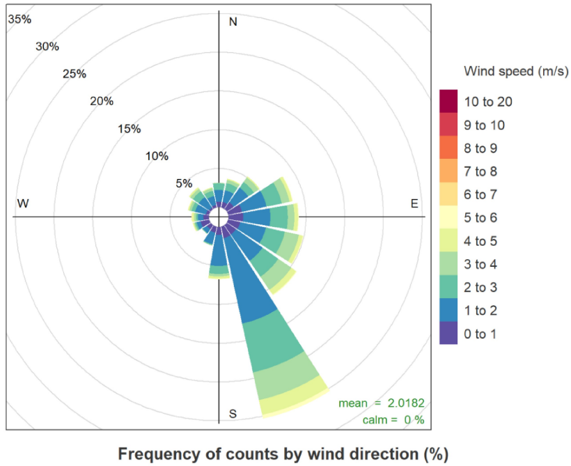
Figure A1 Annual distribution of winds at the Project site predicted by TAPM/CALMET
