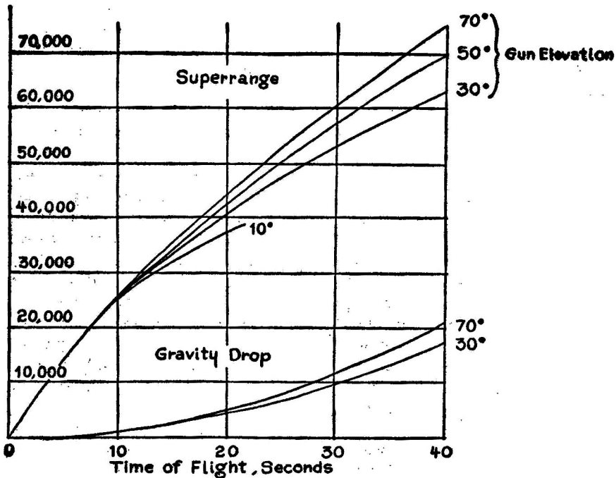
FIG. 4: BALLISTIC DATA
