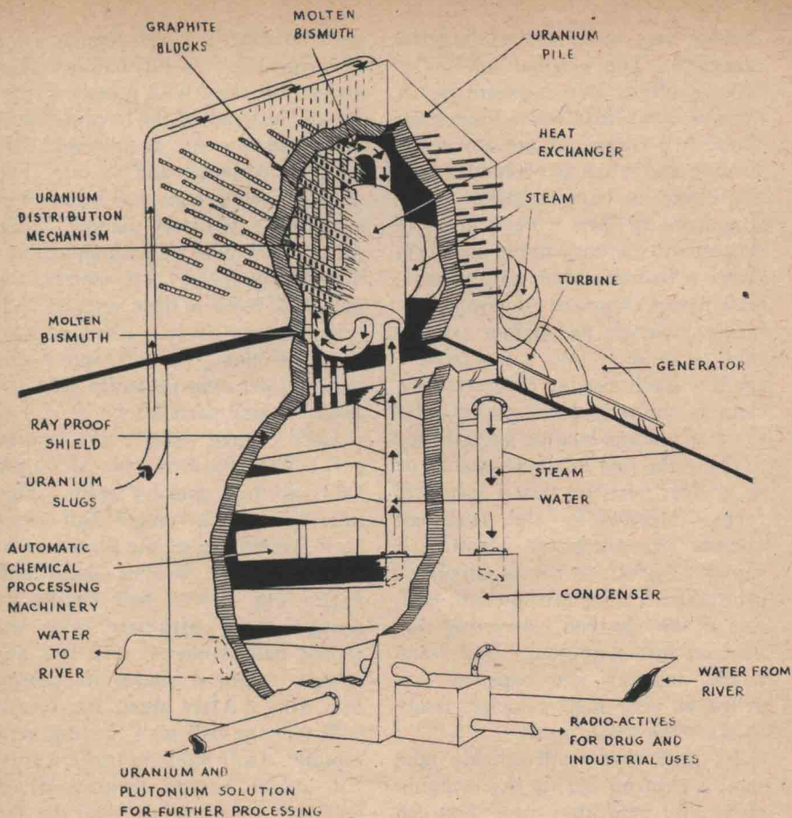
General cutaway diagram of the structure of the atomic power plant proposed on the cover. Rods projecting from the pile are neutron-absorbing control rods. Both automatic, motor-driven, and separate manually operated emergency rods would be installed.
