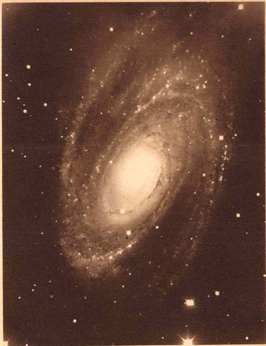
The spiral nebula Messier 81 in Ursa Major. Photographed March 21, 1917, by G. W. Ritchey with the 60-inch Mount Wilson reflector. Ritchey's work with this instrument, which he constructed, was remarkable due to his enormous interest in securing the smallest, sharpest possible images.
