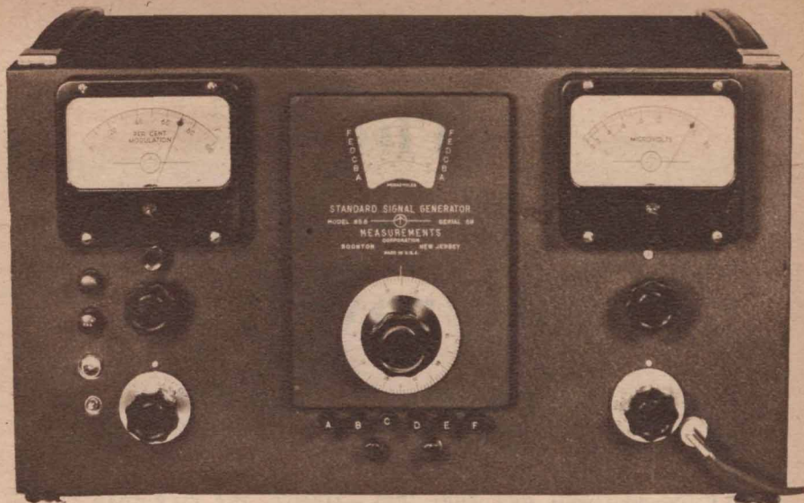
Standard signal generator of the type used for development of home radio receivers, covering frequencies from 75 kc to 39 mc. This particular type combines the "Adjust Meter" and "Microvolts" slide; the upper right knob is the control, the right meter reads the signal level. The left-hand meter and controls handle the audio-frequency modulation. See Fig. 6.
