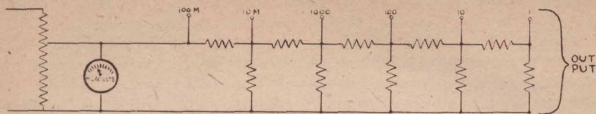
Fig. 6. In other types of Standard Signal Generators, a single slider is used, meter now reading actual voltage applied across the attenuator system input. Output will then be the selected fraction of the meter reading.
