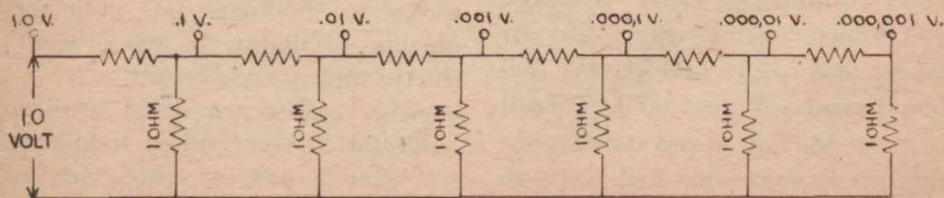
Fig. 4. A ladder attenuator set up so that a tap-switch could pick up one-tenth divisions all the way from 1.0 volts to 0.000001 volt.
