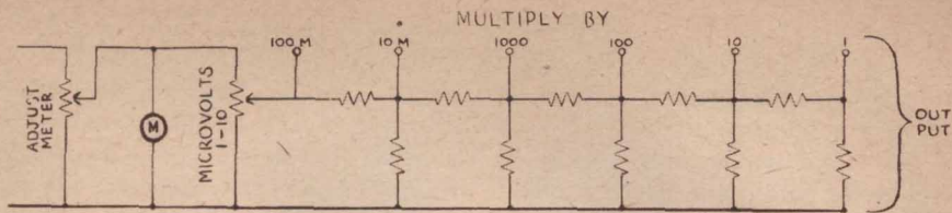
Fig. 5. In Standard Signal Generators, the ladder attenuator is preceded by a slide adjustment. In this "Adjust Meter" type, the meter is set to a predetermined point. Then the second slider will read in microvolts
