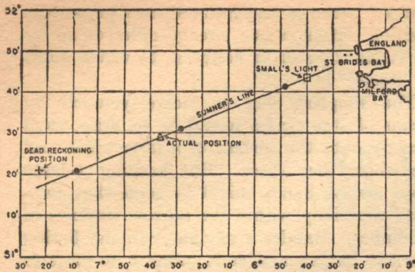
Figure 1 Chart showing the position of Sumner's ship when the "line of position" was first used in navigation.
