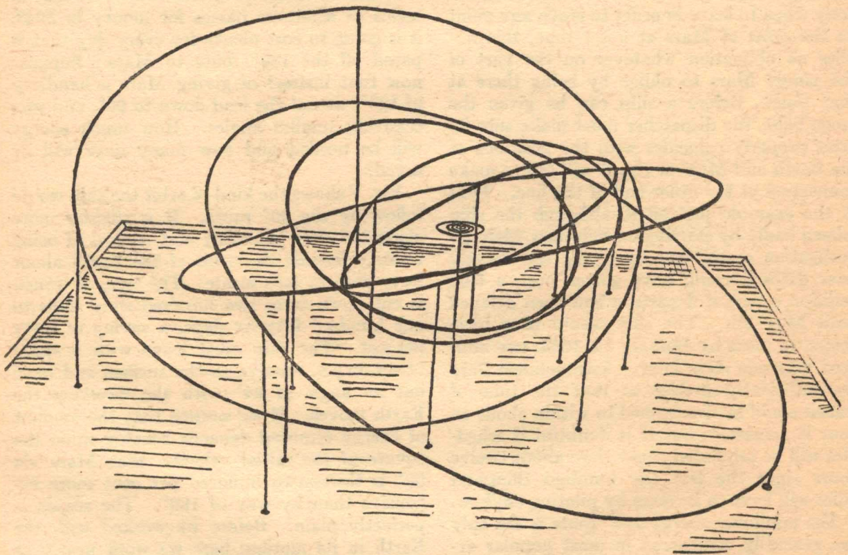
FIG. VIII. Model showing satellite system of Jupiter in perspective. After penetrating six outer orbits would come to the four large Galilean satellites and close inner moon (Jup V). Since five inner satellites revolve in plane of Jovian equator could most easily avoid by landing in high latitude. Rod supporting inner satellites points "up" or toward the north pole of the ecliptic.
