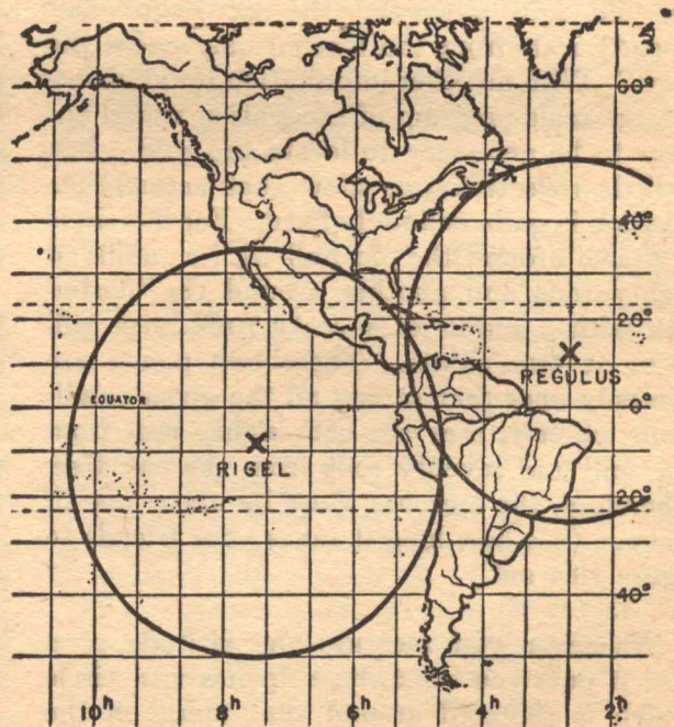
Figure 2. Circles of position from observations of two stars. The substellar points are indicated by crosses. The position of the ship was latitude 17° N, longitude 5 hours 10 minutes west. The position in South America indicated by the other intersection was obviously not that of the ship. The circles are slightly distorted because they are drawn on a projection map rather than on a world globe.
