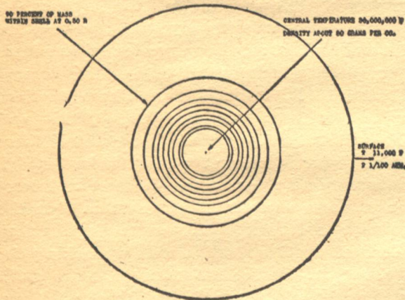
EDDINGTON'S STANDARD MODEL ENERGY IS PRODUCED UNIFORMLY THROUGHOUT STAR THE EQUAL STARS IN MASS
