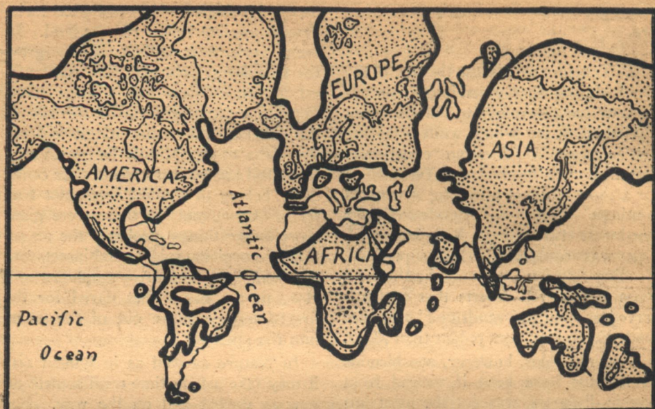
Early Tertiary Period, about fifty million years ago. Today's map is about ready, but more water than ever.
