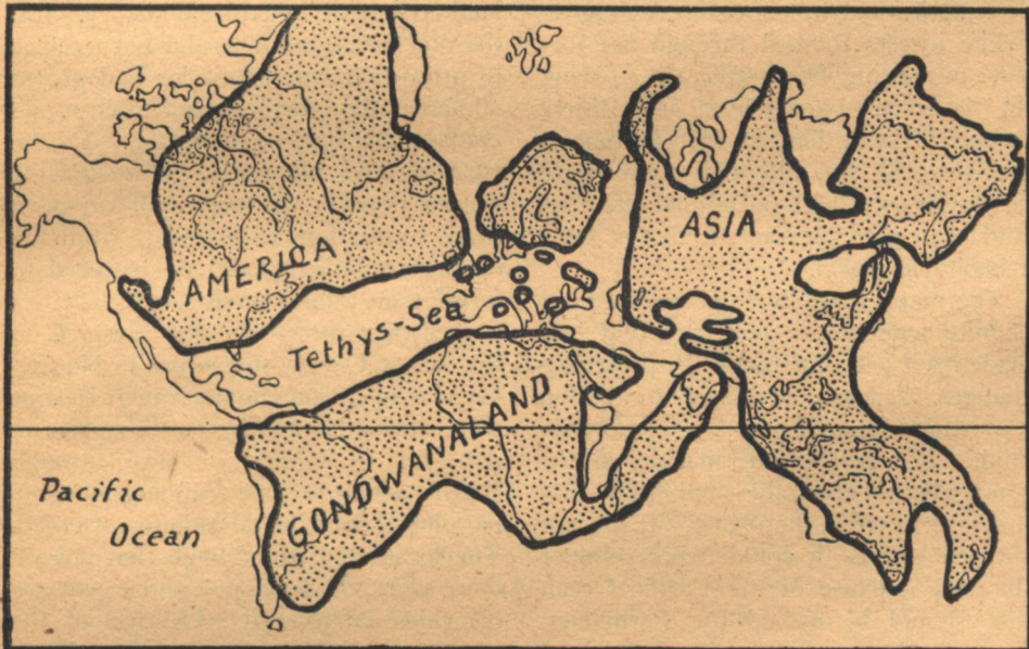
Upper Jurassic Period, about one hundred and thirty million years ago. End of Gondwanaland, the present map begins to shape up.
