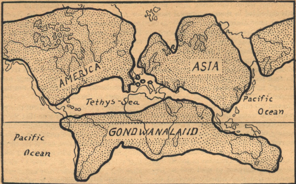
Early Triassic Period, about two hundred million years ago. Period of smallest ocean area on Earth.
