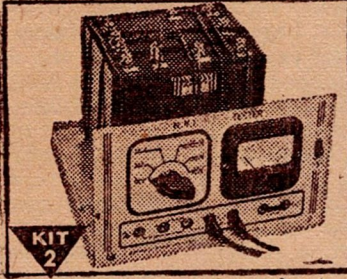
KIT 2 Early in my course I show you how to build this N.R.I. Tester with parts I send. It soon helps you fix neighborhood Radios and earn EXTRA money in spare time.
